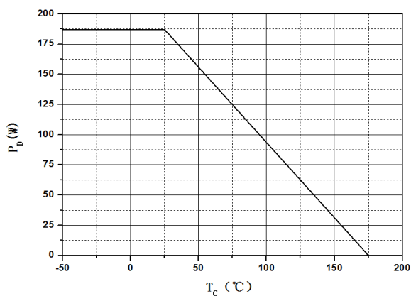
P D VS temperature (TO-263/TO-220C)
