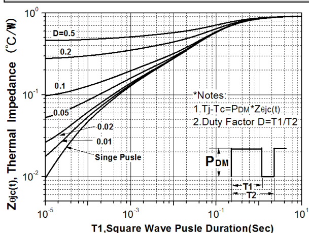
Normalized Maximum Transient Thermal Impedance for IGBT(TO-263/TO-220C)
