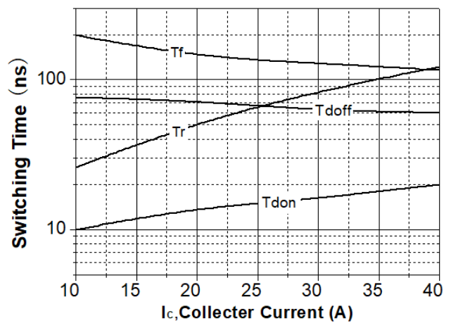
SwitchingTime vs. I_C
